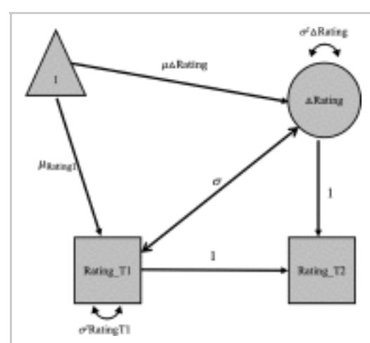
Figure 2 The basic univariate LCS model, with the commonly used symbols in SEM. The variable ‘Rating’ represents severity ratings and is measured at two time points (Rating_T1 and
